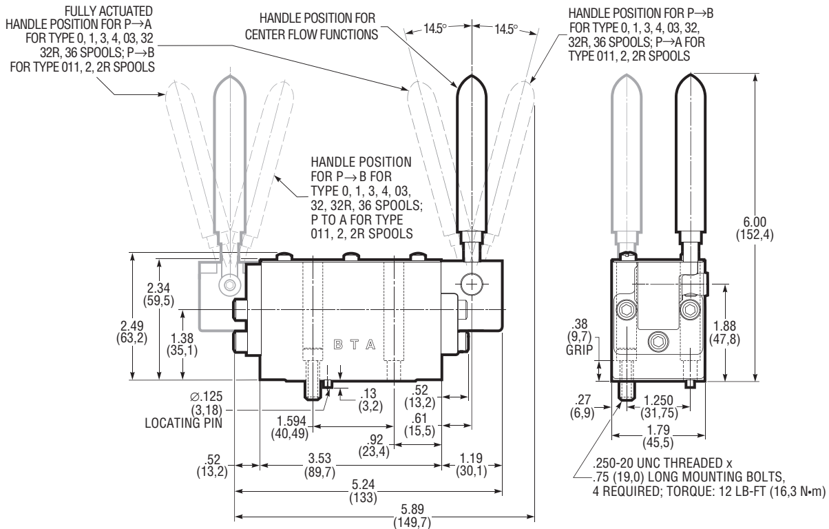
6100 Series, Manual Lever Operated
