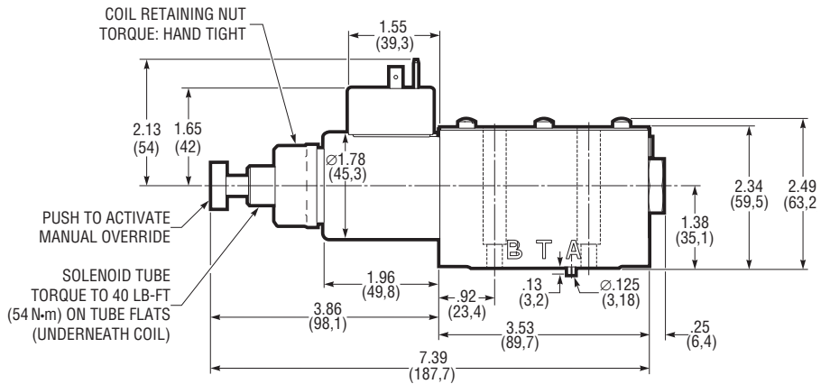
6500 Series, Single Solenoid Models (A.C. DIN Connector Version Shown)
